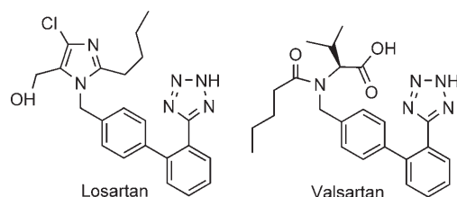
Scheme 1. Sartans.
